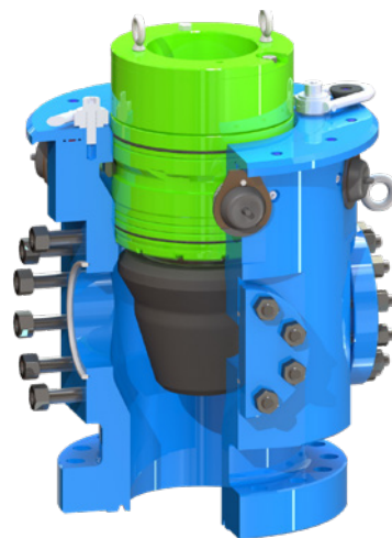
Model T3000 Rotating Control Device (RCD)
